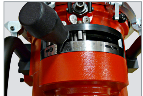
Wachs innovative AutoFeed system allows you to set your desired weld profile with hands-free machining.
