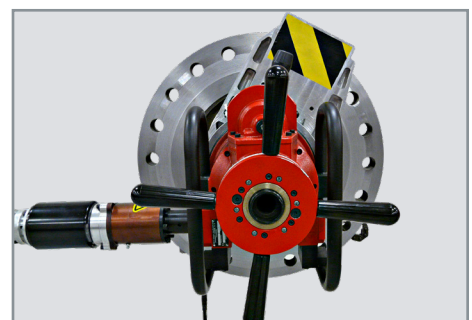
Hydraulic, electric or pneumatic drive options are available. Wachs EP 424 is ideal for flange facing.
