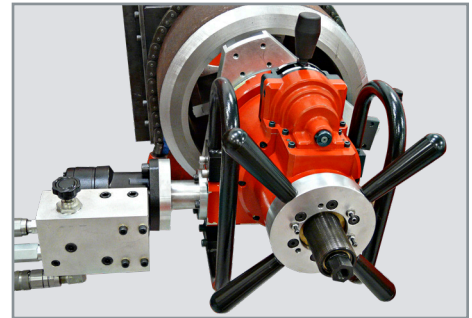
Single point model includes Wachs AutoFeed system. Form tool basic model also available.
